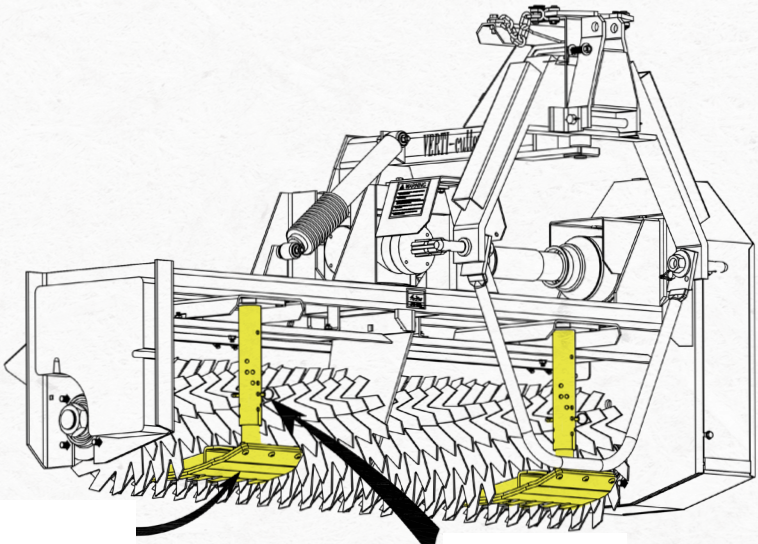
Skid shoes extend between blades for consistent cutting depth over uneven turf
