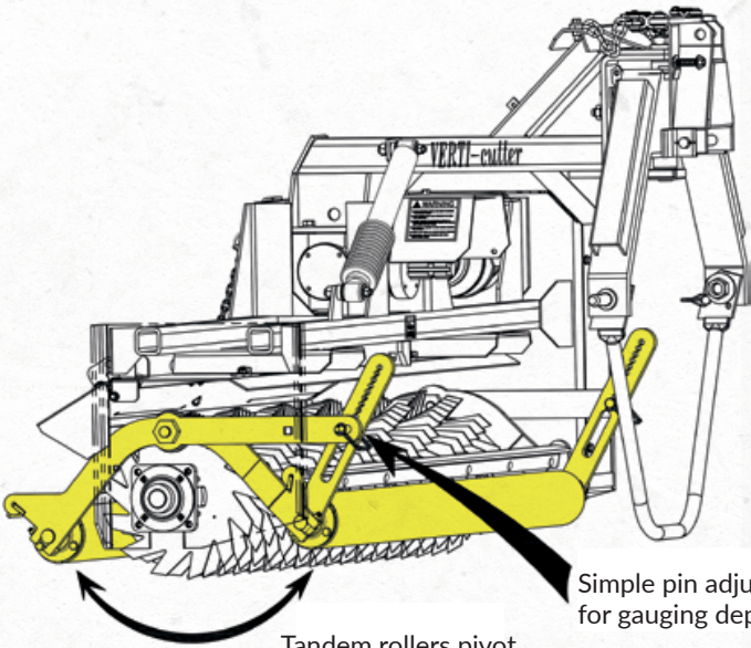
Tandem rollers pivot around blades for consistent cutting depth
