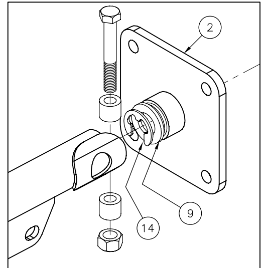
DETAIL C
