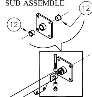
DETAIL C
